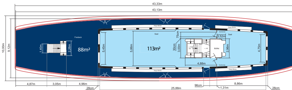
Oberdeck
